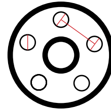
Ford 5 Stud (Only 10" Brakes)
