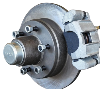
Hydraulic Disc Brake
