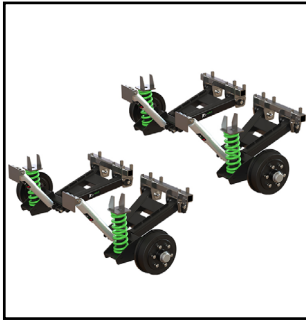
WIS2.8TT 2800KG Rating Tandem
