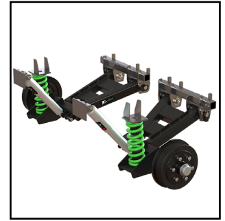
WIS1.6TS 1600KG Rating Single
