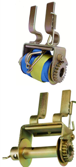
* Clip on Winch with and without strap
